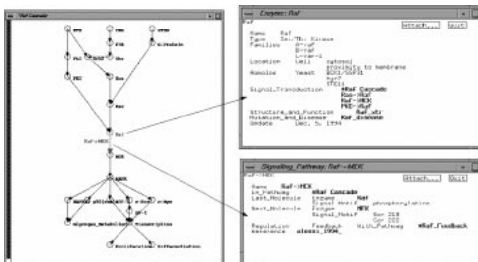
Figure 2: Examples of signal pathway diagram (left) and its corresponding deeper information (right).
